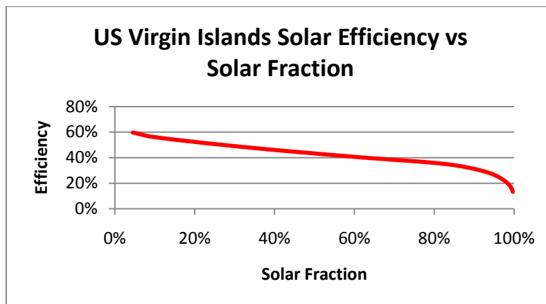
Figure A-15. General trend of SWH efficiency versus SF
