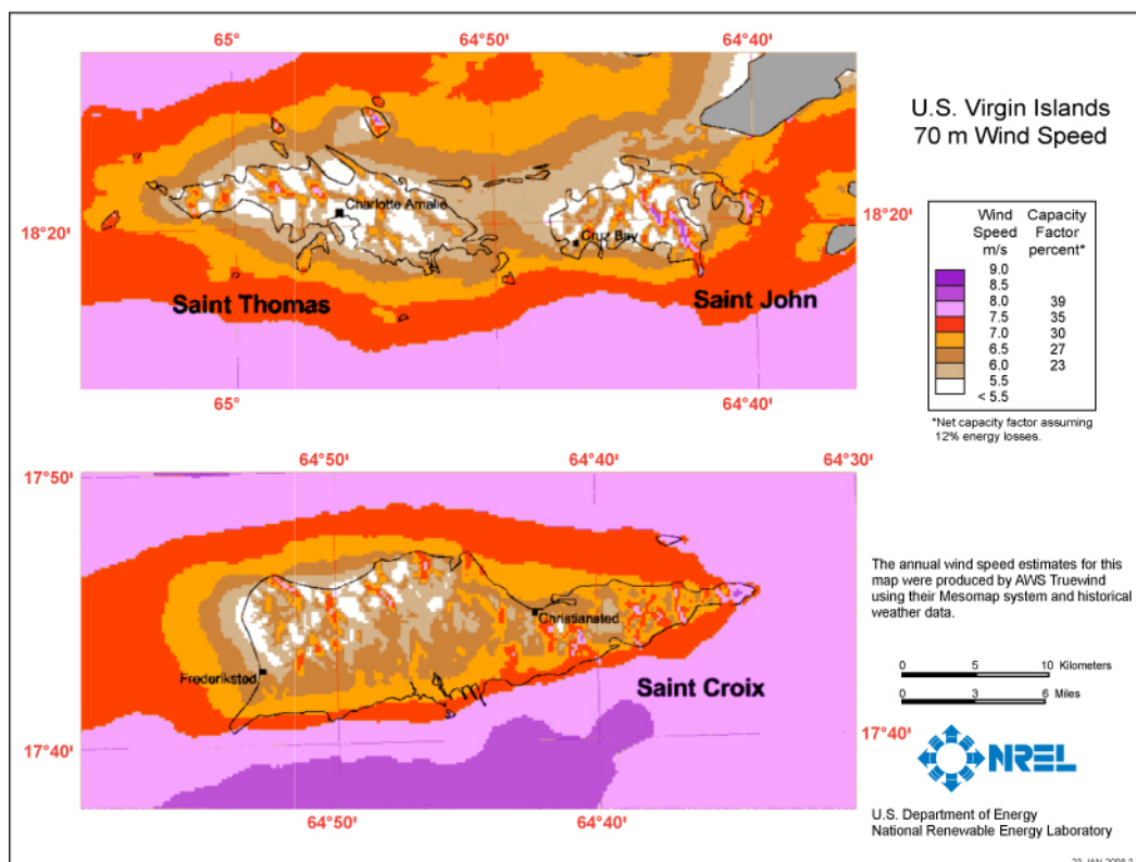
Figure 21. Estimated annual wind speeds for the USVI
