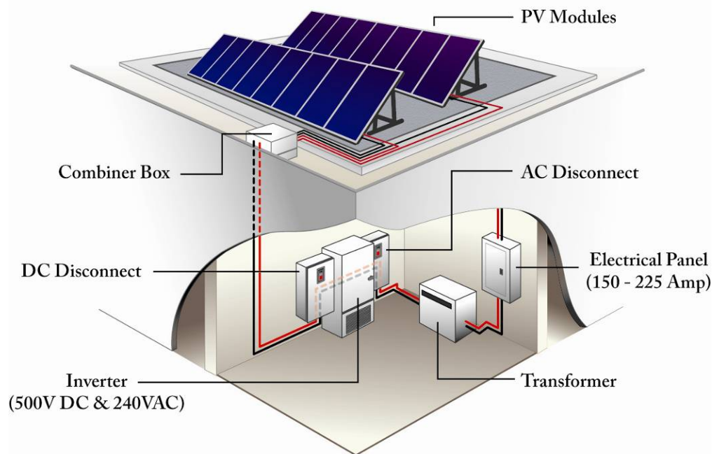
Figure A-10. Photovoltaic system schematic
