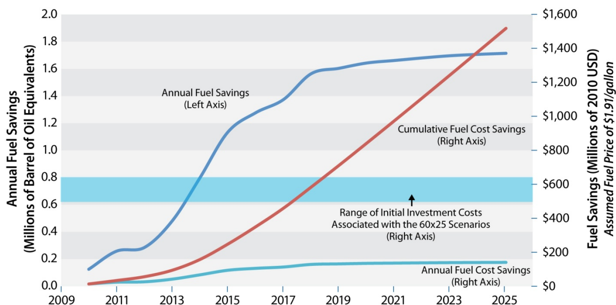
Figure 26. Expected fuel savings in barrel of oil equivalents, cost savings at $1.91/gal, and capital expenditures required to achieve 60x25
