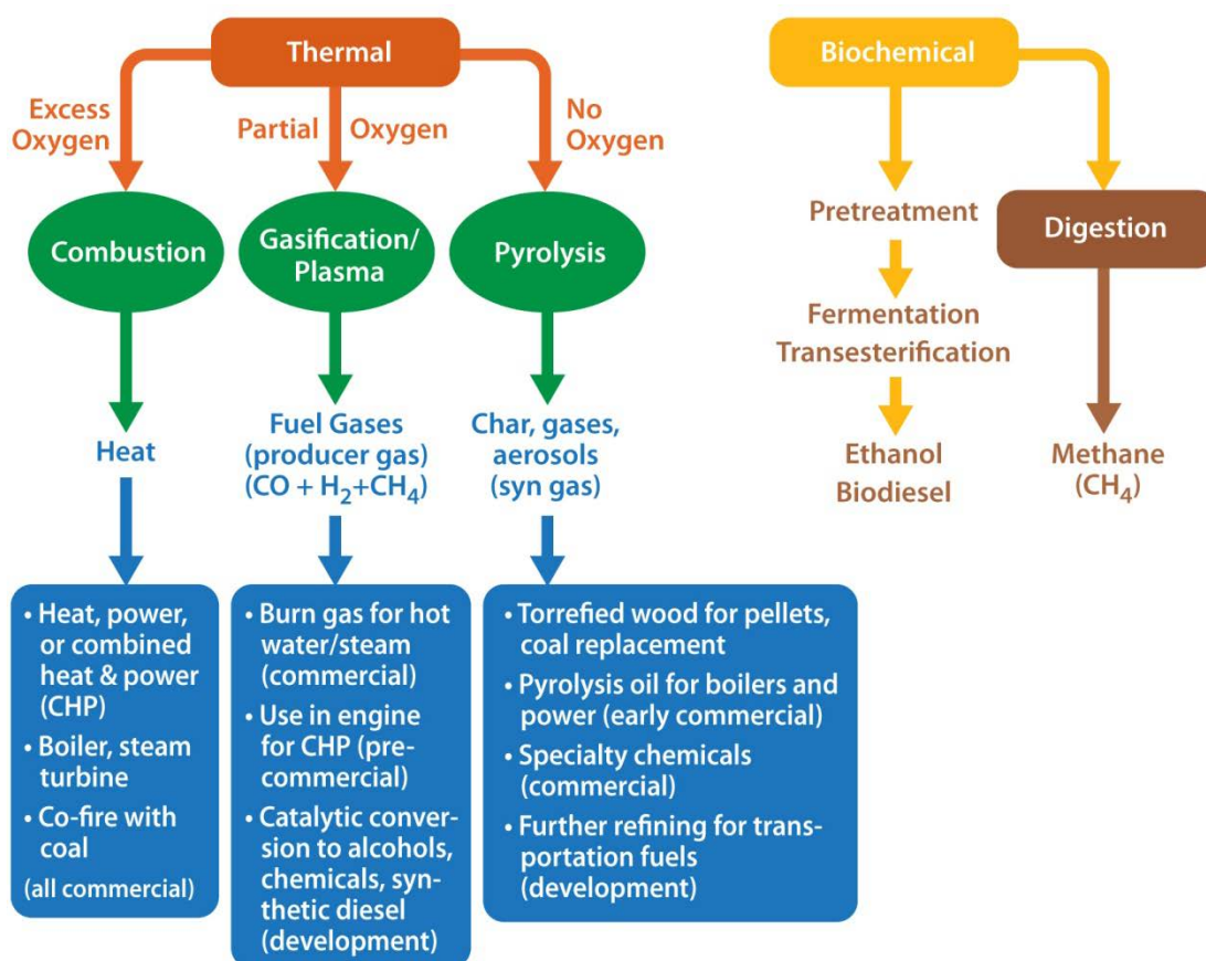
Figure 19. Waste-to-energy conversion pathways
