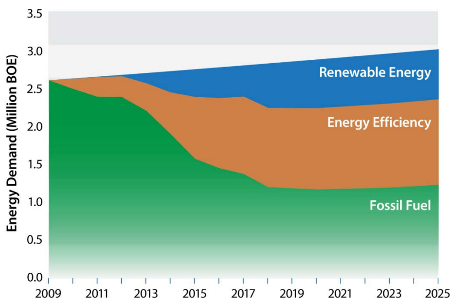
Figure 10. Base case energy mix in the USVI, 2009–2025
