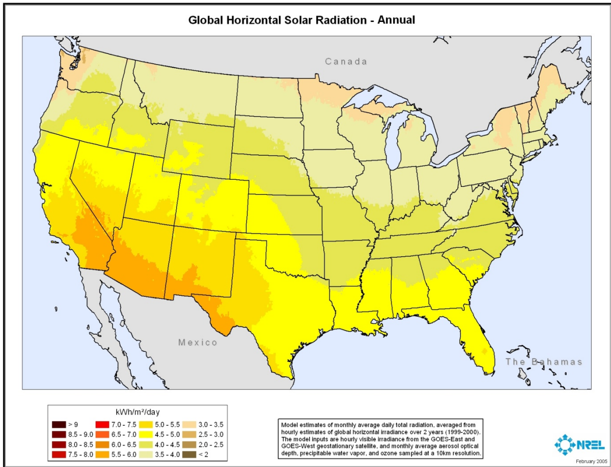
Figure A-12. U.S. total solar resource
