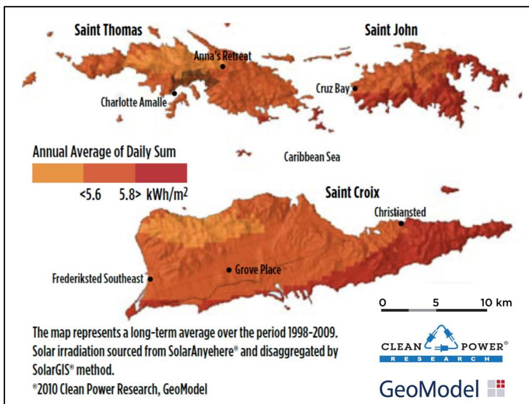
Figure 16. USVI solar resource map Illustration from Clean Power Research
