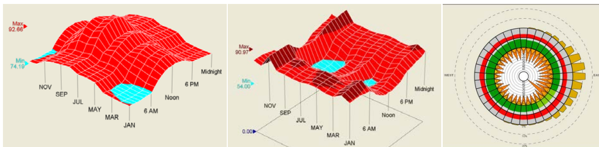
Figure B-1. Annual temperature, humidity, and wind profiles
