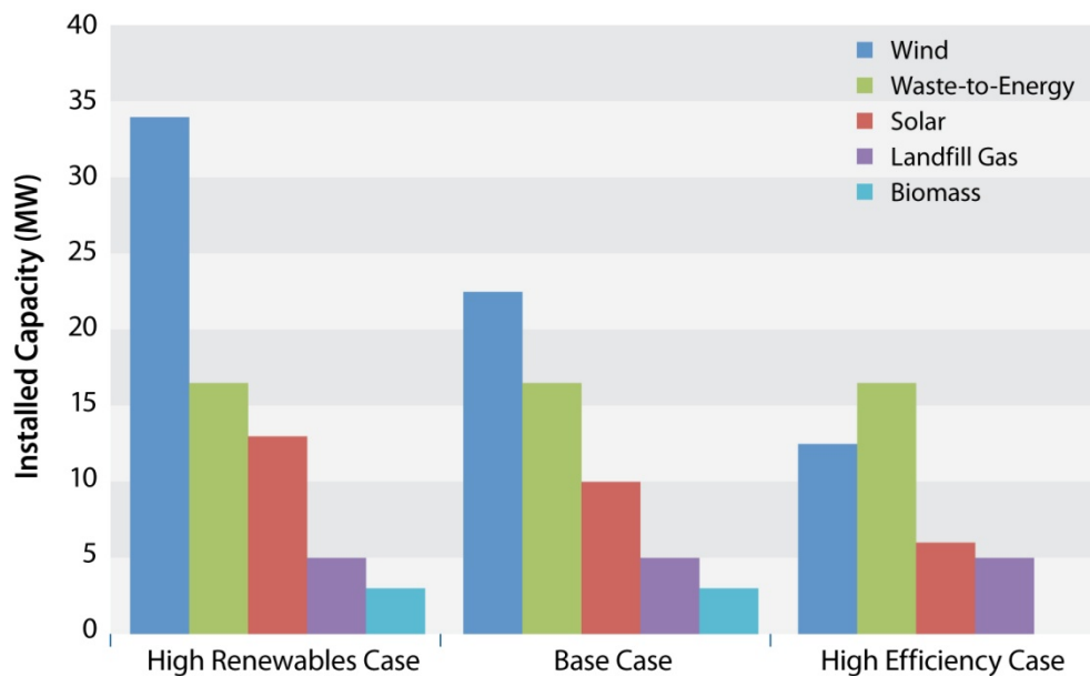
Figure 29. Deployment of renewable power generation technology across scenarios
