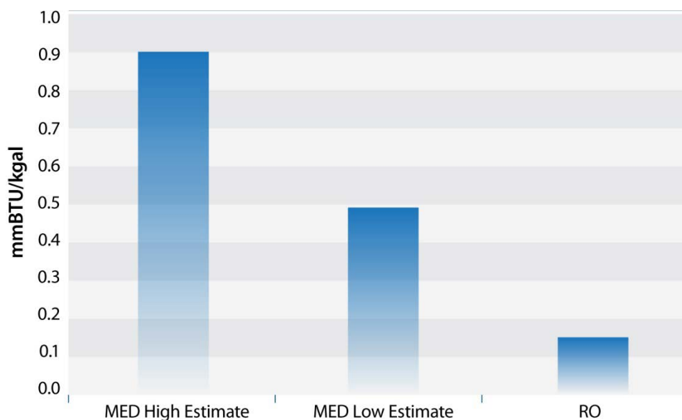
Figure 13. Energy use for desalination—MED versus RO
