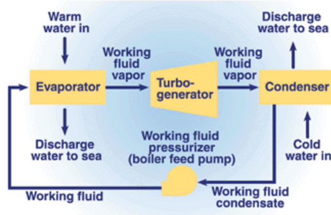
Figure A-8. Closed loop cycle OTEC
