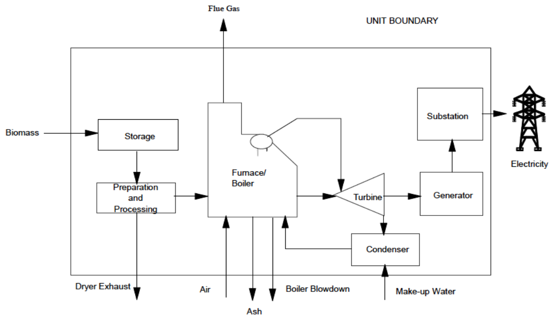
Figure A-1. Direct-fired biomass
