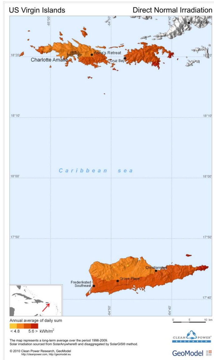
Figure A-6. Direct normal radiation estimates for the USVI
