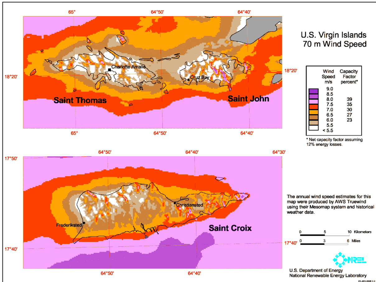
Figure A-16. Wind resource potential in the USVI at 70 m
