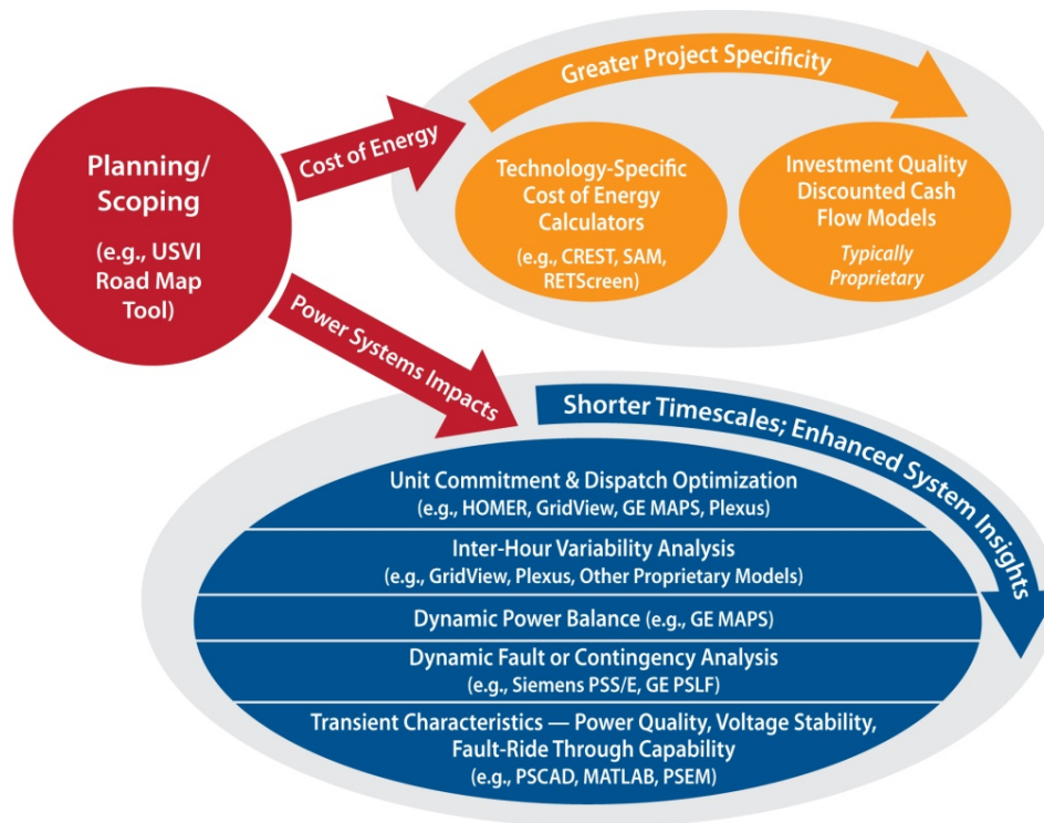
Figure 7. Analytical planning and optimization tools
