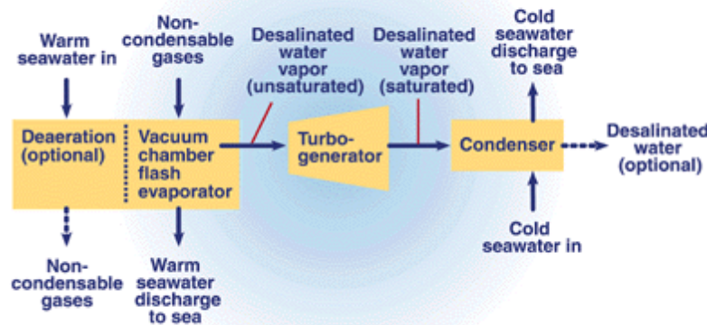
Figure A-7. Open loop cycle OTEC
