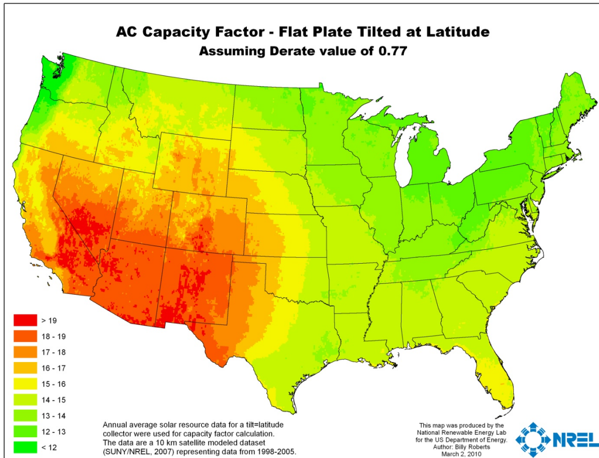
Figure A-11. PV system performance by region
