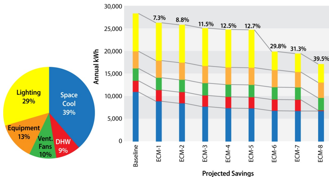
Figure B-6. Energy end-use and savings potential—3,000 ft 2 , with air-conditioning
