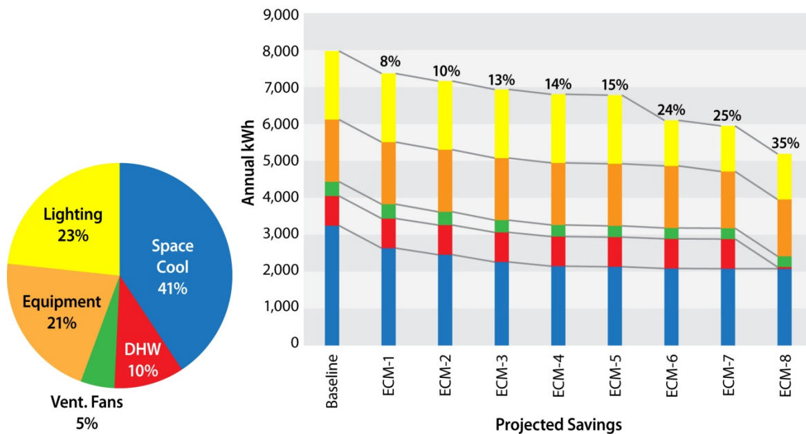
Figure B-5. Energy end-use and savings potential—900 ft 2 , with air-conditioning
