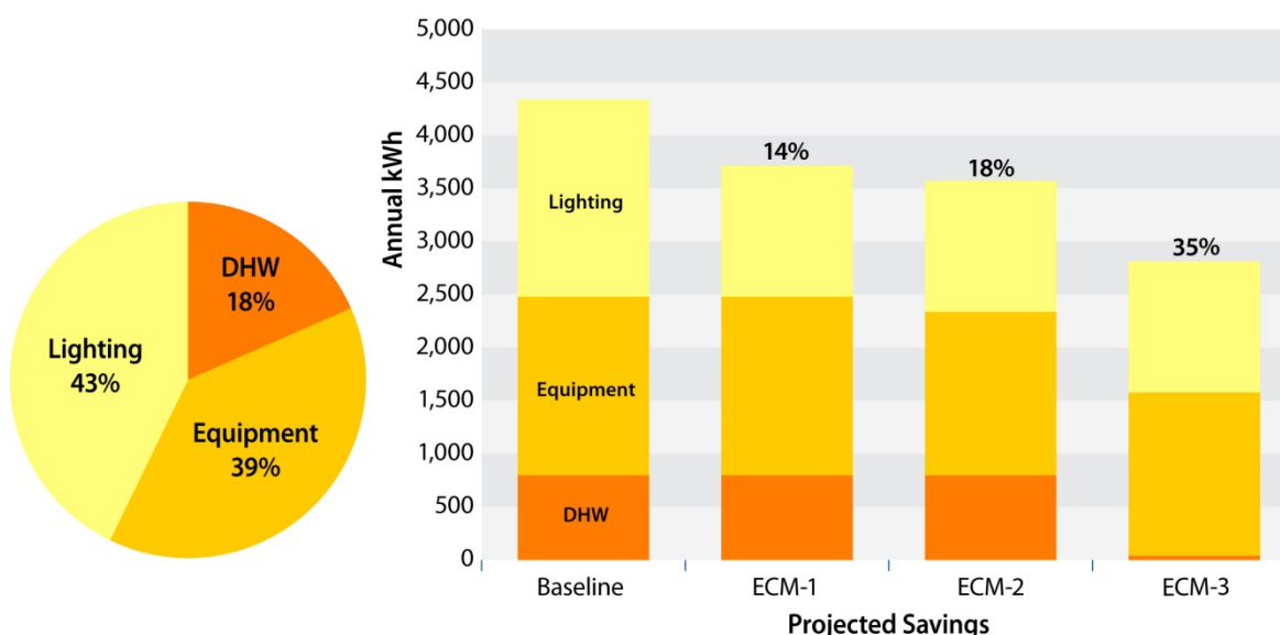
Figure B-4. Energy end-use and savings potential—900 ft 2 , no air-conditioning
