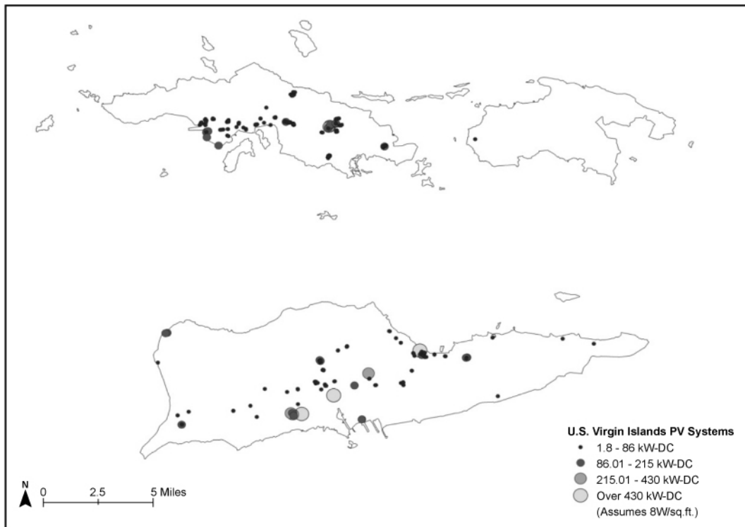
Figure 17. USVI potential PV system sites
