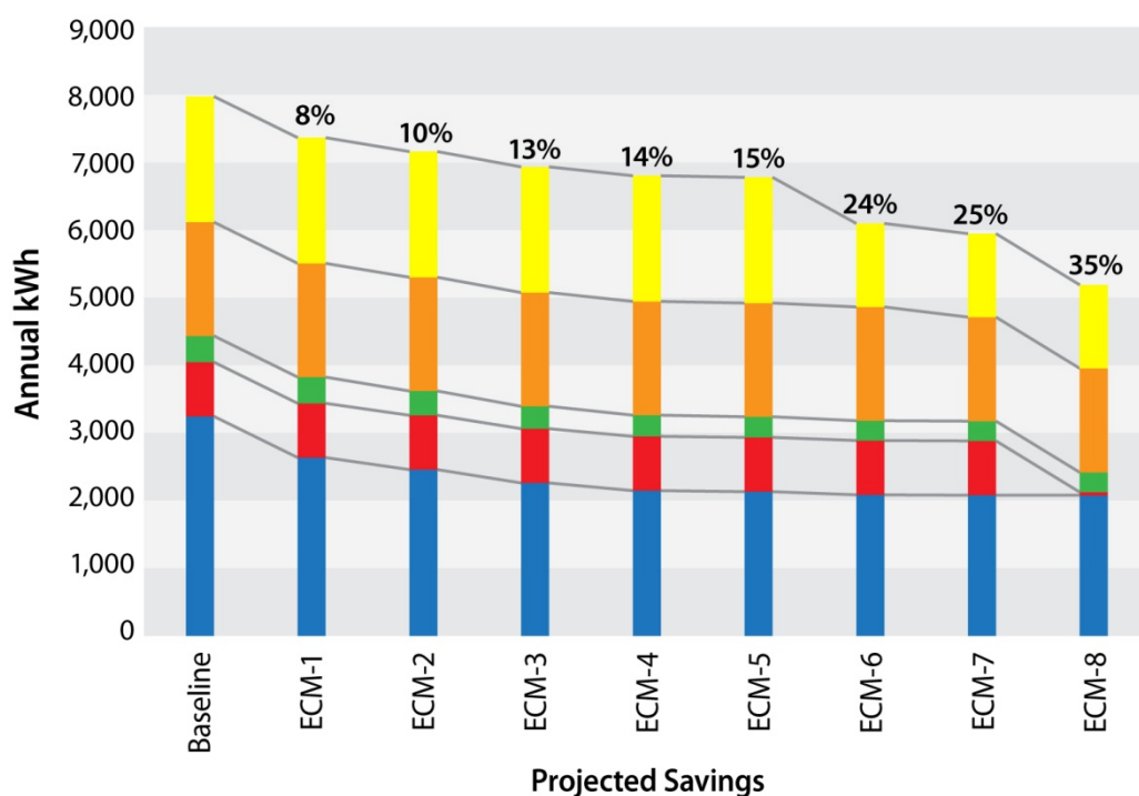
Figure 15. Impact of individual energy conservation measures in a typical 900 ft 2 home with air-conditioning
