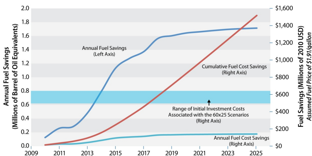
Figure ES-1. Expected fuel savings in barrel of oil equivalents, cost savings at $1.91/gal, and capital expenditures required to achieve 60x25
