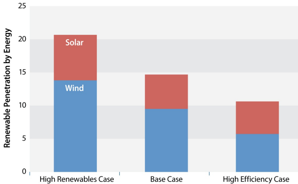
Figure 30. Average penetration by energy of variable output renewables on the USVI grid across scenarios
