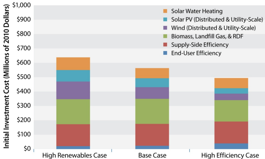
Figure 28. Estimated initial investment costs to deploy the technology utilized in each scenario
